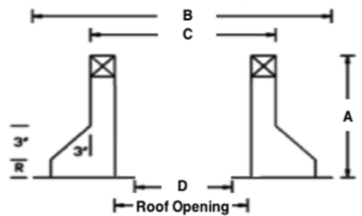
Raised Canted Curb (RCC)
