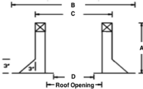
Canted Curb (CC)
