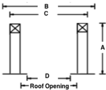
Straight Curb (SC)
